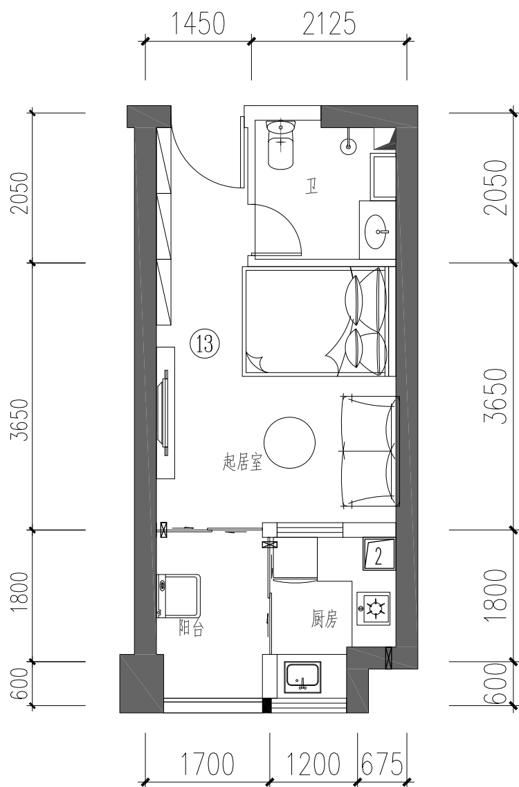
02/05/08/13户型平面图
